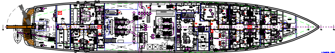
LOWER DECK
