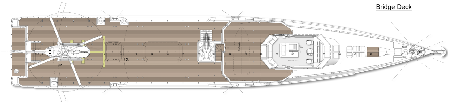
Main Deck
