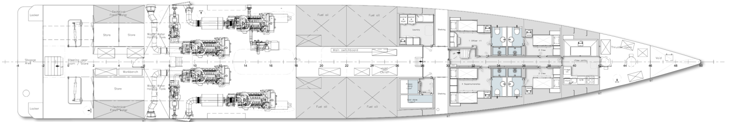
Lower Deck
