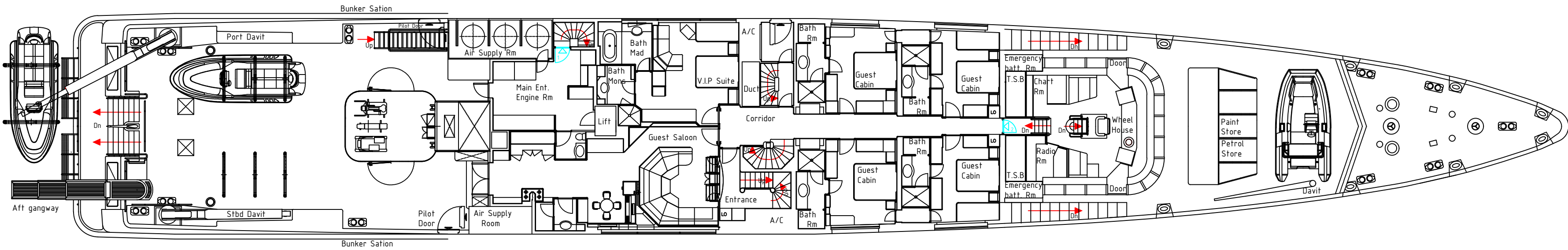
LOWER DECK
