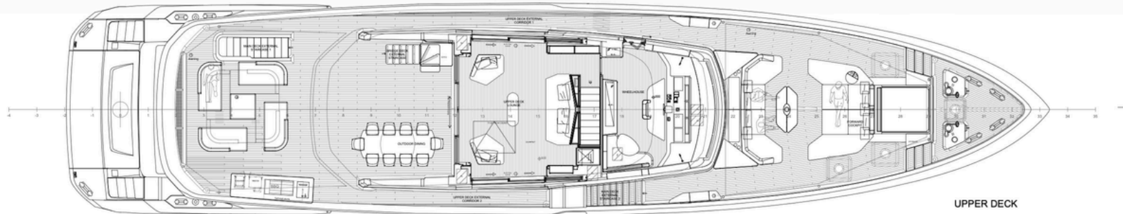
UPPER DECK
