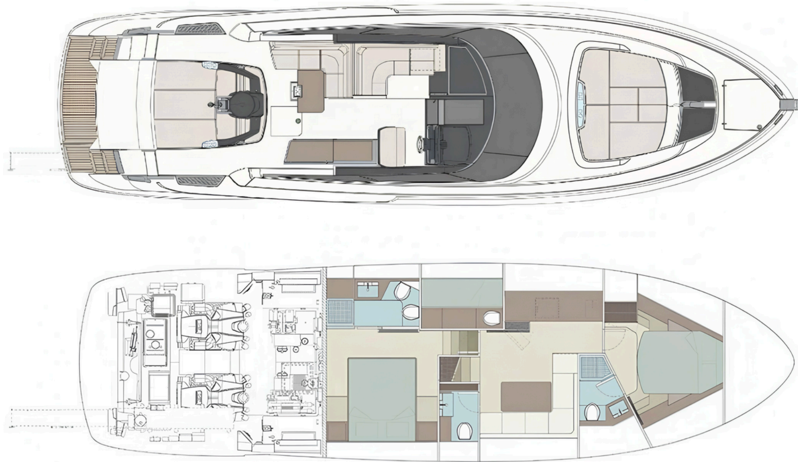
GENERAL ARRANGEMENT
